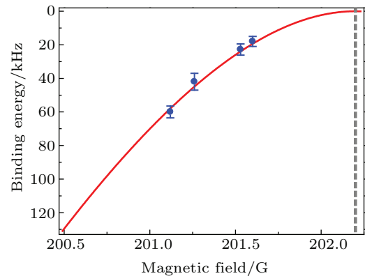
Fig. 3. (color online) Binding energy of weakly bound molecules versus the external magnetic field. The blue error bars are the binding energies of the molecules in experiment, and the red solid line is the theoretical calculation.
